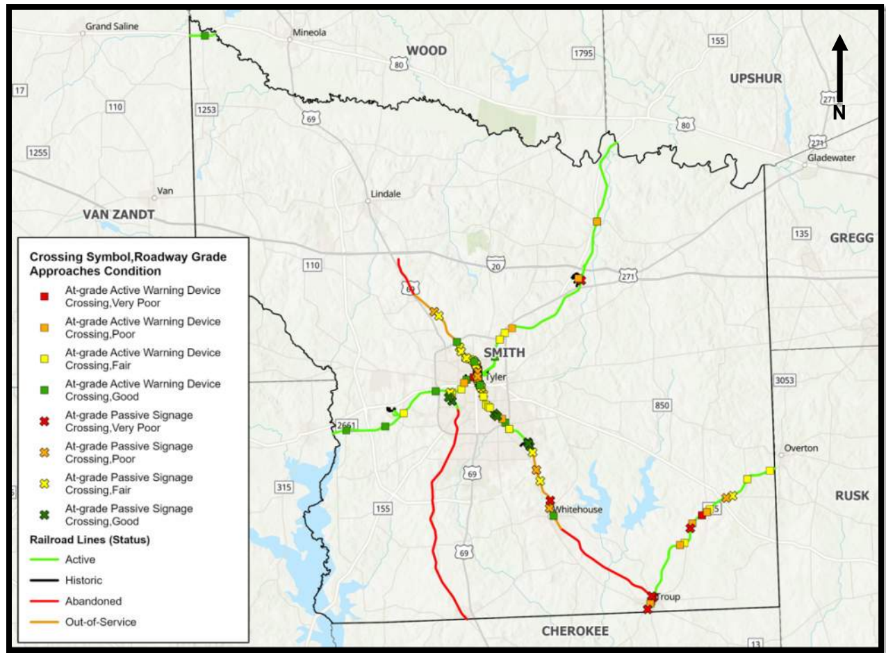
Figure 13: Roadway Grade Crossing Approaches Condition Assessment Results
