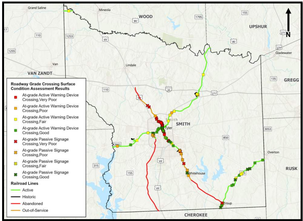
Figure 12: Roadway Grade Crossing Surface Condition Assessment Results
